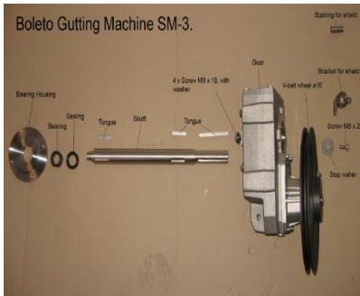
K-1068: complete set replacement gear for SM3 – see page 7 details
