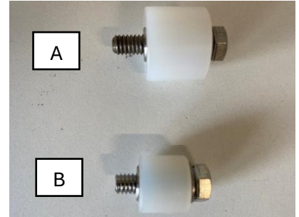
K-1055: Roll with shaft (slitting element) big (A) + small (B)
